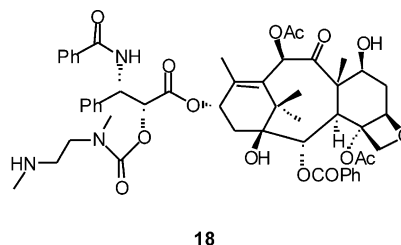
Figure 6. Structure of intermediate 18 .
