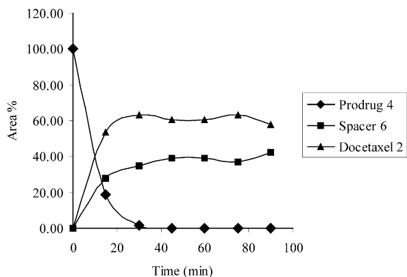
Figure 3. Enzymatic cleavage of prodrug 4 .
