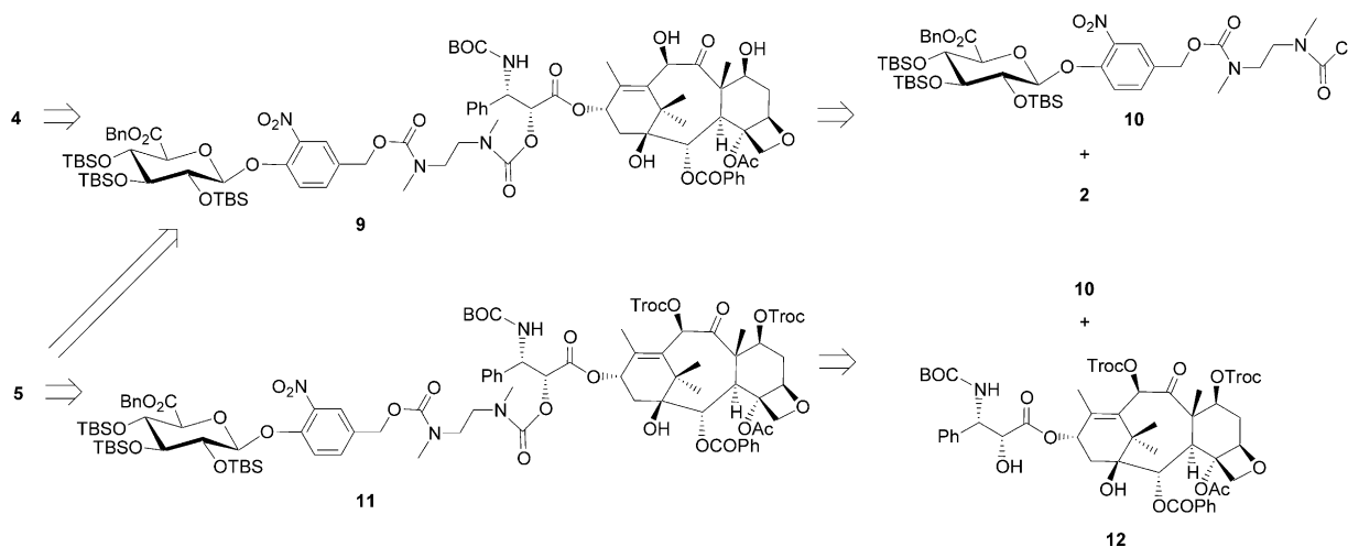
Scheme 2. Retrosynthetic scheme of compounds 4 and 5 .
