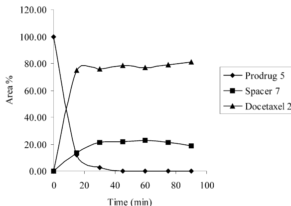
Figure 4. Enzymatic cleavage of prodrug 5 .
