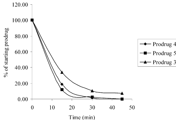
Figure 5. Comparison of the disappearance of the three prodrugs.
