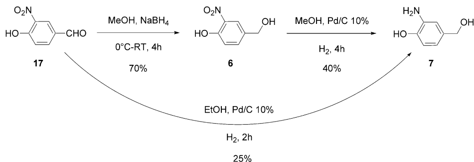
Scheme 5. Synthesis of spacers 6 and 7 .
