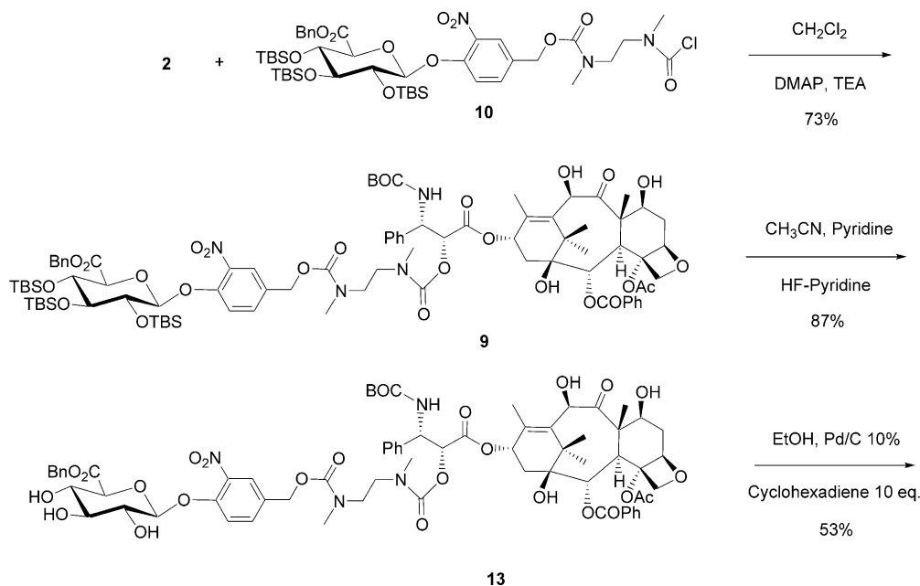
Scheme 3. Synthesis of prodrug 4 .
