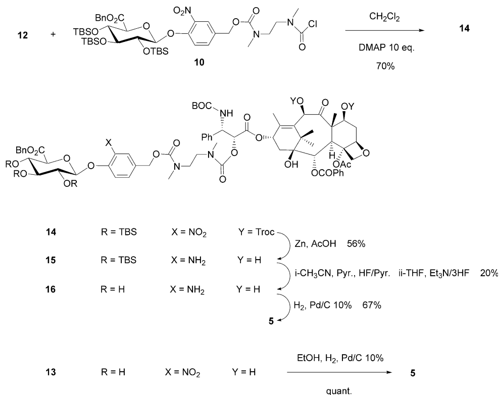
Scheme 4. Synthesis of prodrug 5 .
